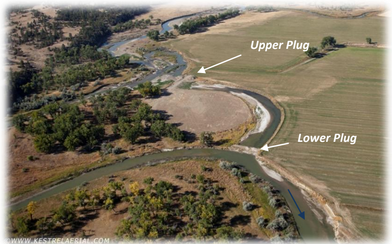
Figure 4. View upstream of plugged avulsion.
